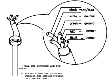
WIRING- SCHEMATICS FIXTURE-5WIRE FEED 0-10V DIMMING
