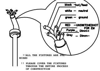
WIRING- SCHEMATICS FIXTURE-6WIRE FEED 0-10V DIMMING AND EM
